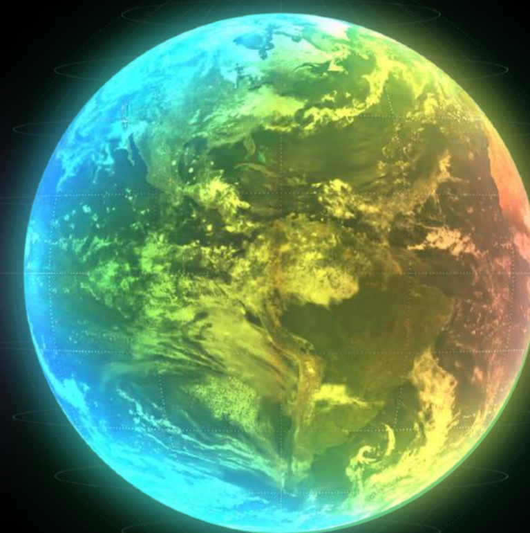
THERMOSPHERIC DRAG
